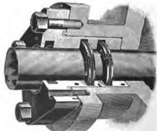
Fig. 1021. Metallic Piston Rod Packing. Aurora Metal Co.
